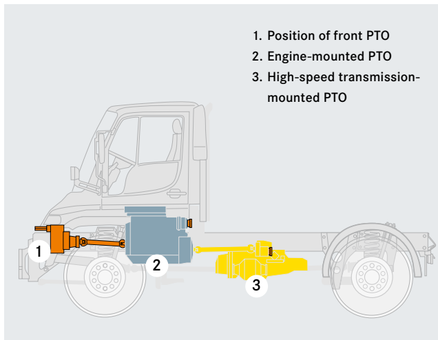
Unimog U 400/U 500: locations of front PTO (1), engine-mounted PTO (2) and high-speed transmission-mounted PTO (3).
